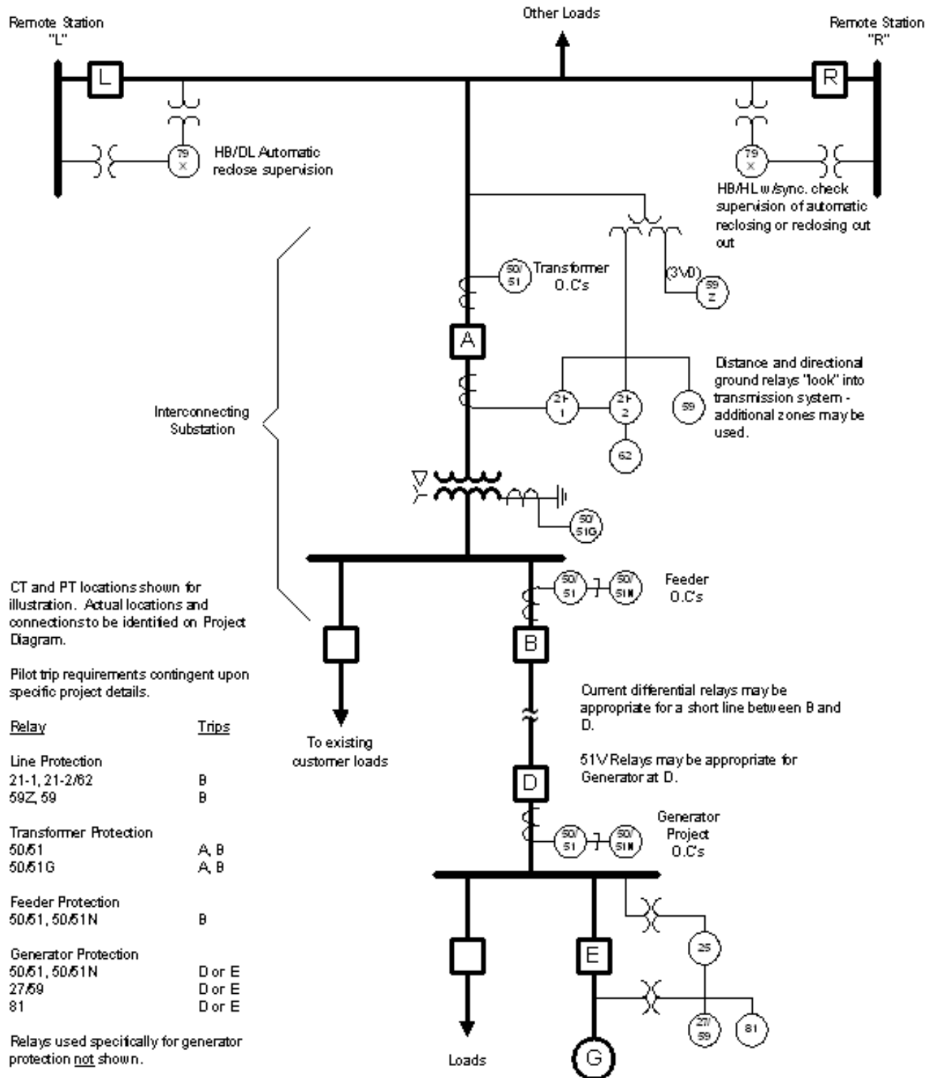
Figure 12.--- Integration of Generation to an Existing Low Voltage Substation Connected to a Transmission line a \Delta -Y \Delta Transformer and Protected by a High Side Circuit Breaker (Switcher)
