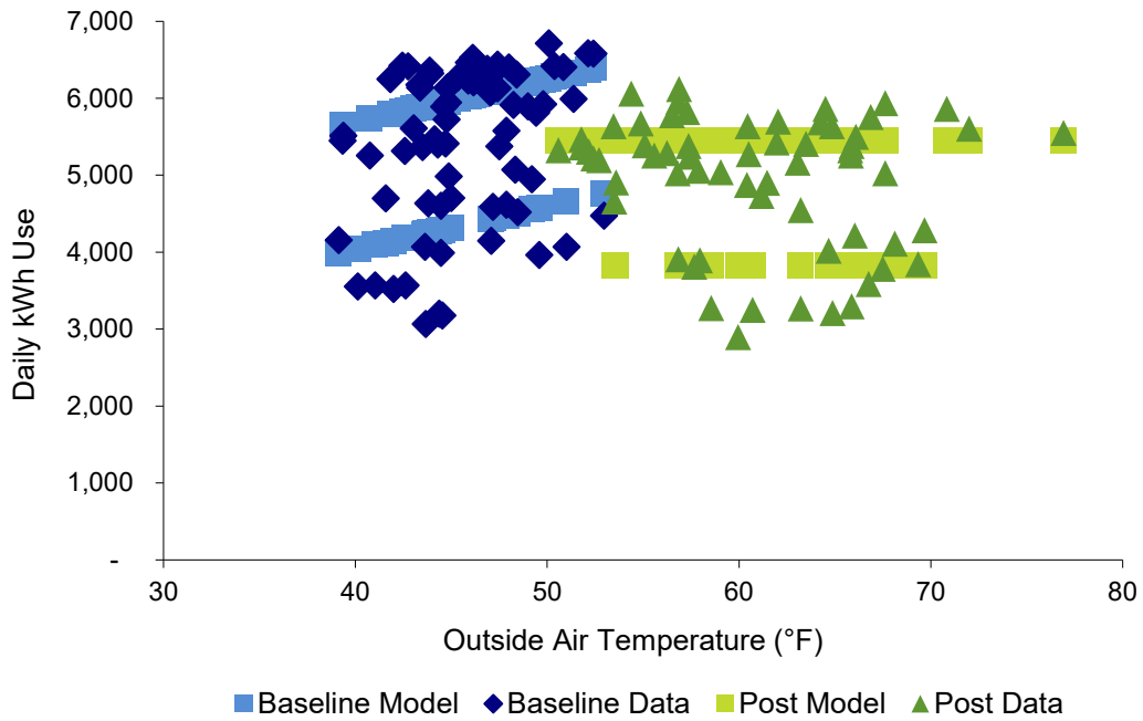
Figure 6-1: Whole Building Electric Data and Model
