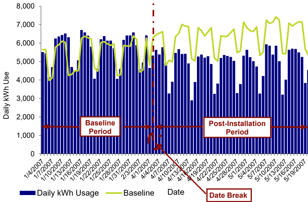
Figure 6-4: Electric Savings Resulting from Retro-Commissioning University Library
