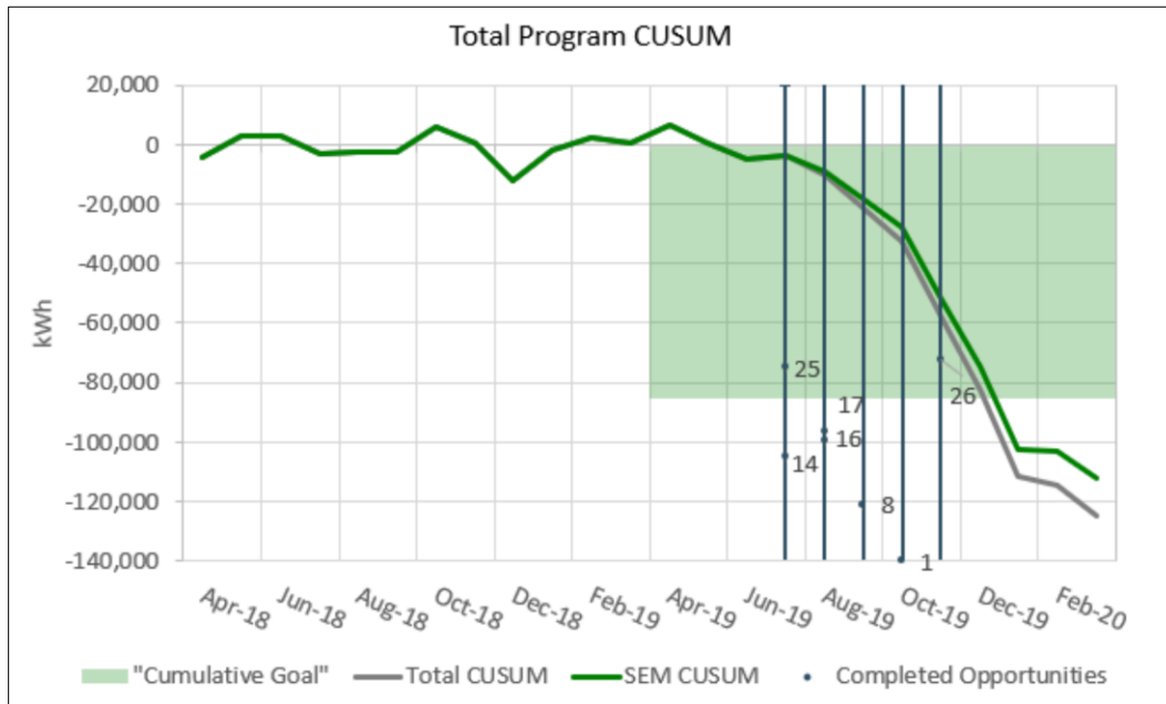
Figure 10-3: Cumulative Sum of Savings Over The Reporting Period
