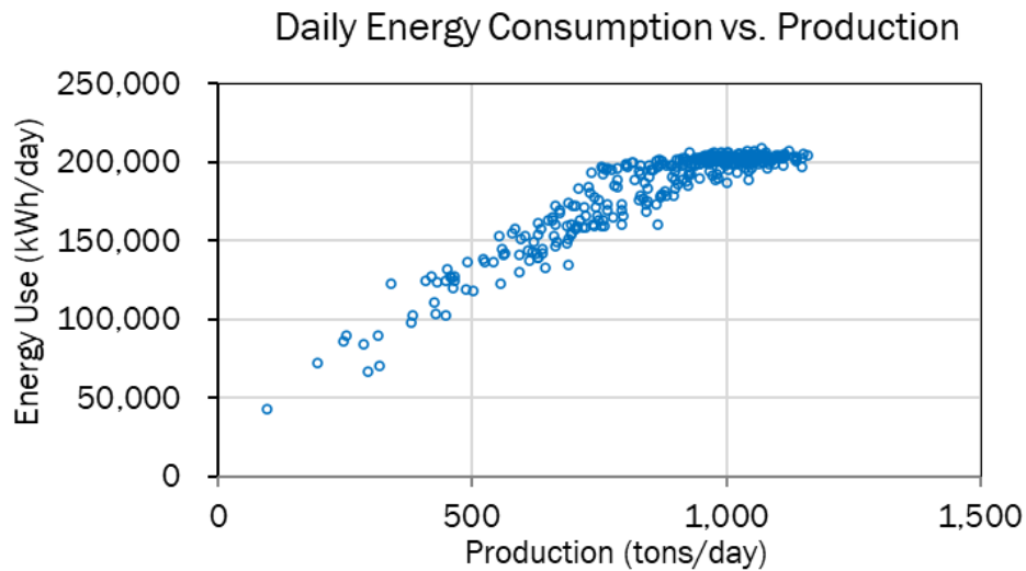
Figure 5. Example Scatter Plot (Energy vs. Production)
