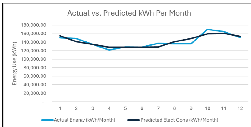
Figure 10-2: Actual vs. Predicted kWh Per Month for Baseline Period
