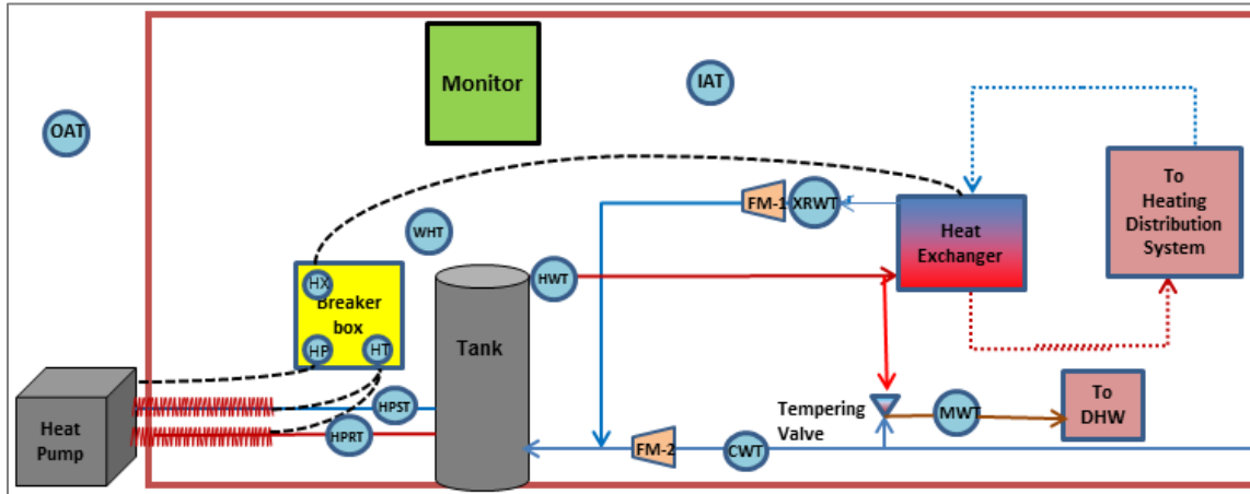
Figure 4. Onset Monitoring Configuration for a Typical Split System
