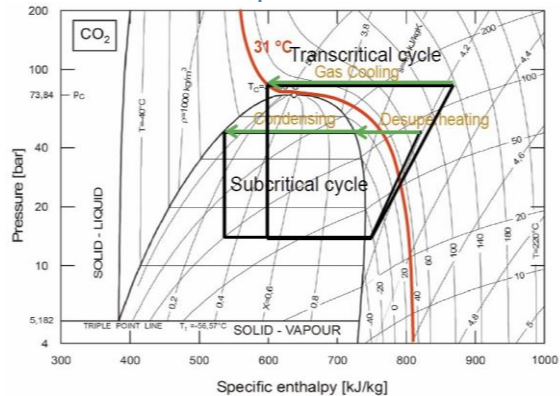
Figure 1. Comparison of CO 2 and Standard Refrigerant Operation
