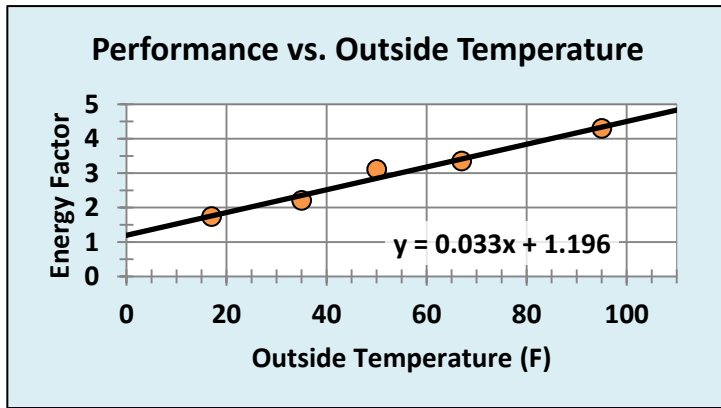
Figure 21. Energy Factor for Various Test Temperatures
