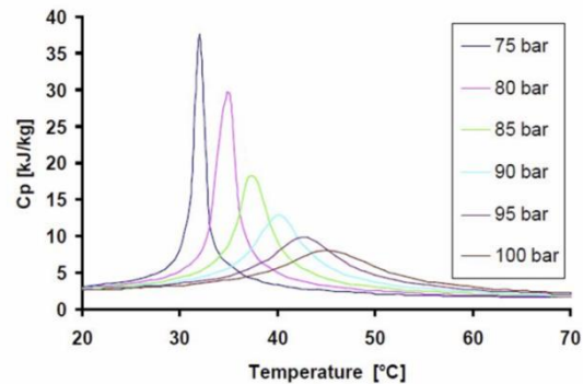
Figure 2. Impact of Operating at Optimum Specific Heat
