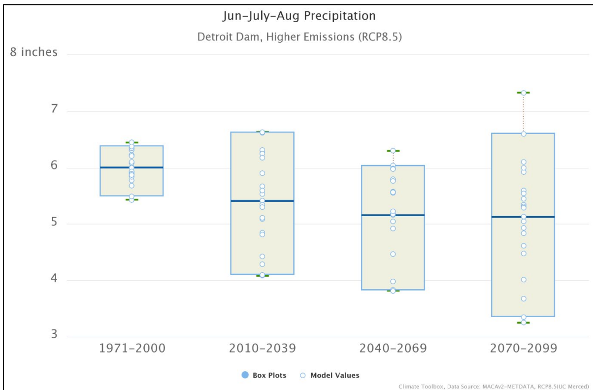
Figure 3-29. Median Summer Precipitation Trends at Detroit, Oregon, 1950–2100.
