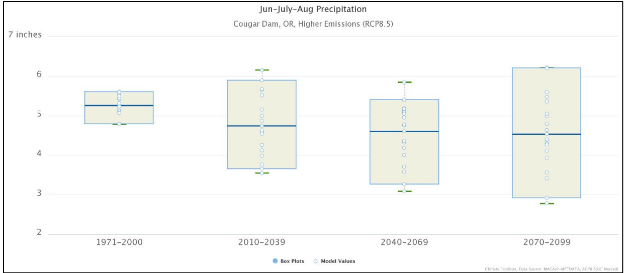
Figure 3-43. Median Summer Precipitation Trends at Cougar Dam, Oregon, 1950–2100.
