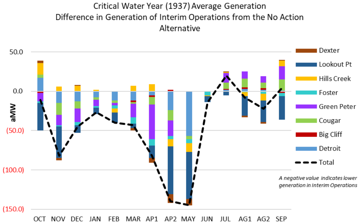
Figure 2.2-16. Critical Water Year (1937) Average Generation: Difference in Generation of Interim Operations from the NAA
