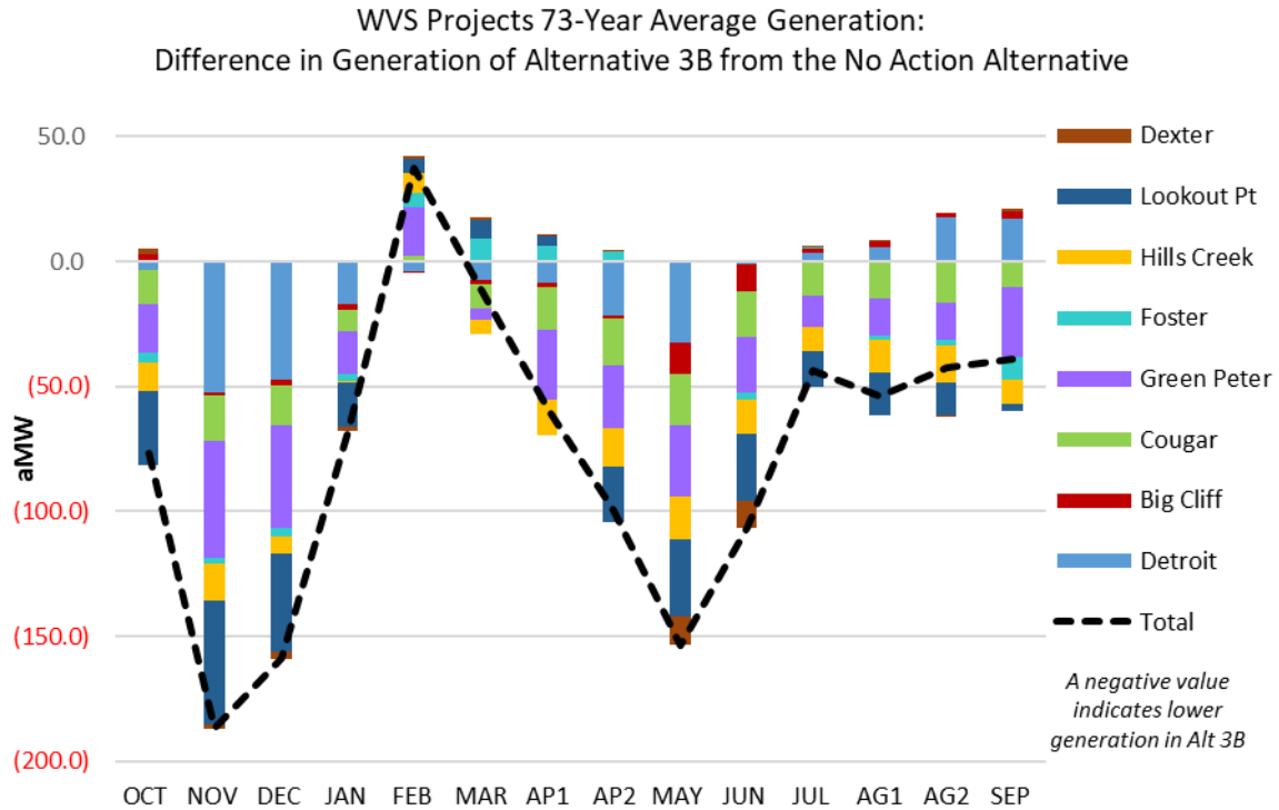
Figure 2.2-11. 73-Year Average Generation: Difference in Generation of Alternative 3B from the NAA
