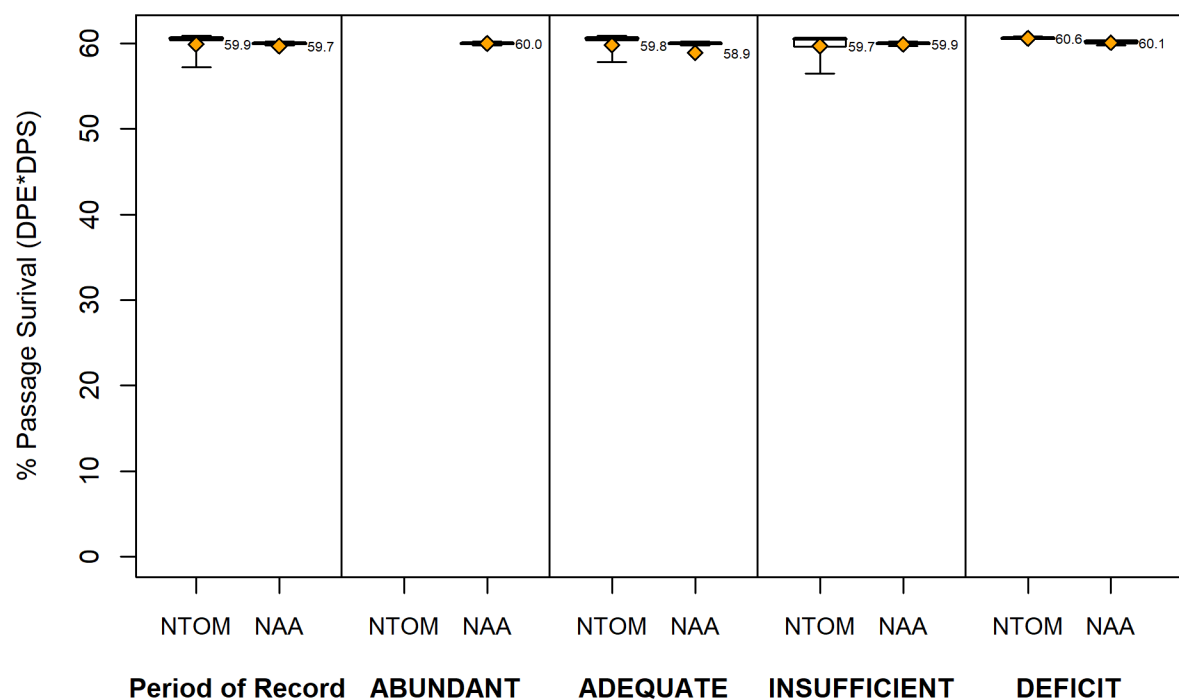
Figure.8_99.Foster.Juvenile.Spring.Chinook.Sub_Yearling.Downstream.Passage.Survival.Under.NTOM;Downstream.dam.passage.survival.at.Foster.for.juvenile.Spring.chinook.sub_yearlings.under.NTOM;The.mean.is.given.by.the.point.estimate.(filled.dot);Survival.probabilities.are.given.for.the.period.of.record.(far.left)?compared.to.abundant?adequate?insufficient?and.deficit.hydrologic.year.types.denoted.in.each.panel;
