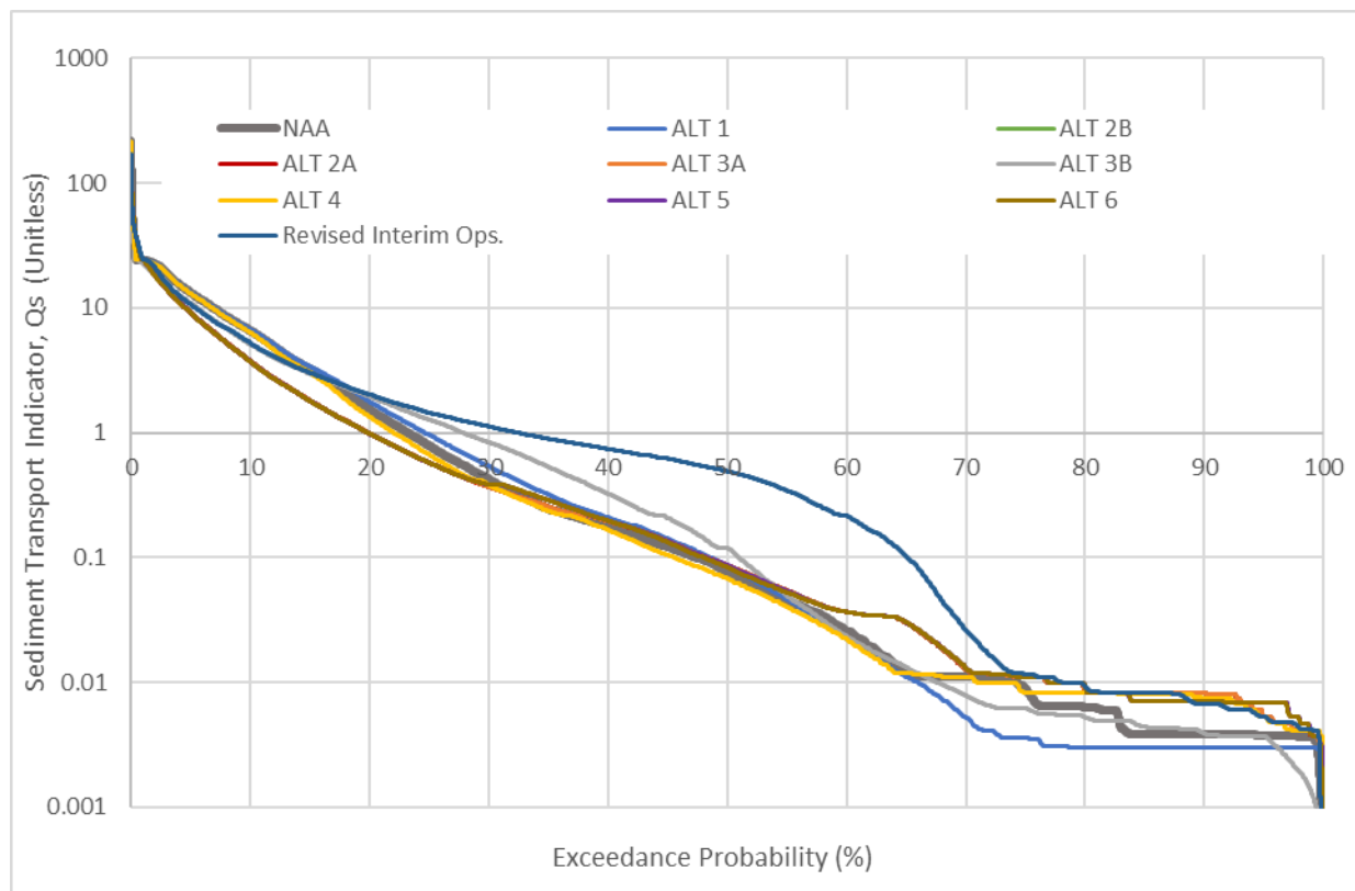
Figure 2-22. Foster Sediment Transport Indicator
