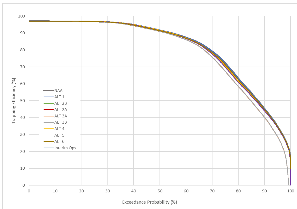
Figure 2-2. Blue River Trapping Efficiency Daily Exceedance
