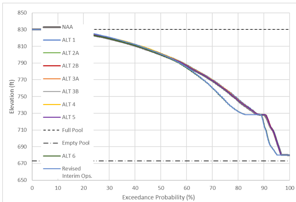
Figure 2-18. Fall Creek Elevation Daily Exceedance
