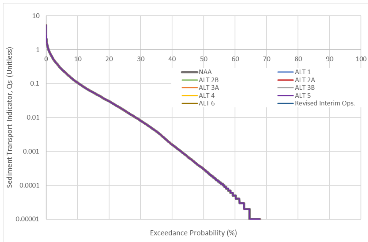
Figure 2-19. Fern Ridge Sediment Transport Indicator
